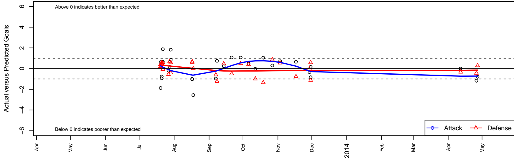
DMS11 Academy B95 Dots are actual minus expected GF (blue circles) and GA (red triangles). Blue line is smoothed change in attack strength. Red is smoothed change in defense strength.
